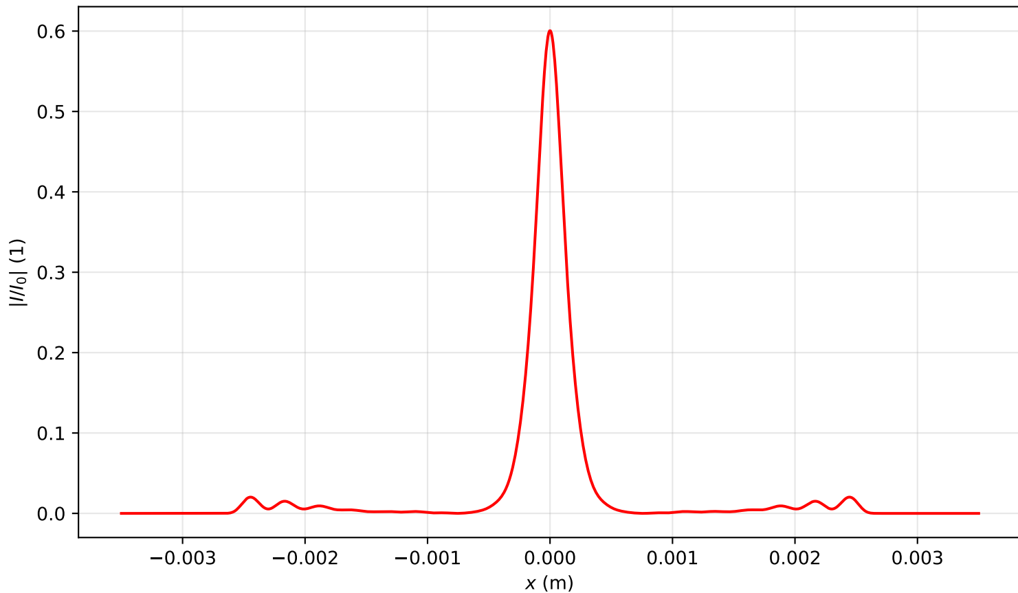
Intensity profile I(x, y = 0, z = 1.911)/I_0 , P_{in}=7.0P_{cr} , artificial time
